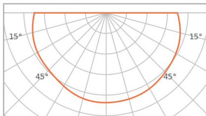
COCO-LPE-9402 - 180° BEAM
