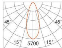
AT 3000K, 90CRI 3000K- 31.8° BEAM
