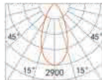
AT 3000K, 90CRI 3000K- 48.5° BEAM
