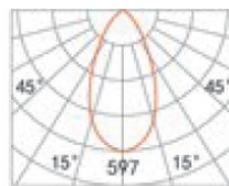
AT 3000K, 90CRI 3000K- 48.9° BEAM
