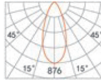
AT 3000K, 90CRI 3000K- 35° BEAM
