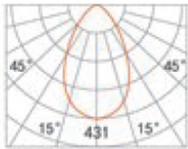
AT 3000K, 90CRI 3000K- 57° BEAM
