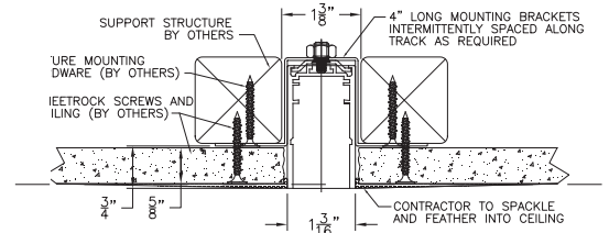
Recessed mud-in installation
