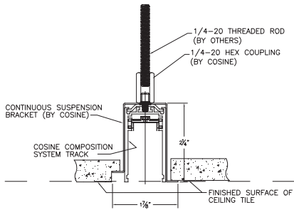
Recessed track in ACT within tile field
