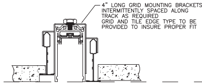
Recessed track in ACT with grid along sides 9/16" suprafine grid 9/16" interlude or slot grid (Left side)
